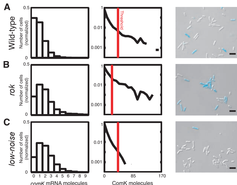
Fig. 4. Noise reduction in comK expression lowers the percentage of competent cells. The leftmost column depicts comK mRNA distributions predicted by the model for the WT (A), and low-noise (C) strains at T_0 . The middle column shows ComK protein distributions at T_0 assuming a high rate of translation in the WT and rok strains [(A) and (B)] and a lowered rate of translation in the low-noise strain (C). The vertical red lines show the predicted threshold beyond which the positive autoregulatory loop of comK would be activated, resulting in competence [the threshold in the rok strain changes because of increased gene expression (see SOM)]. The rightmost column shows CFP fluorescence images from the three strains, taken at T_2 and overlaid on DIC images. All three strains expressed the comK-cfp* fusion, thus fluorescing when competent. The lowest panel in the column shows a microscopic field for the low-noise strain selected to show one competent cell, although the frequency of such cells was less than 1%. Scale bars, 4 \mu m.
