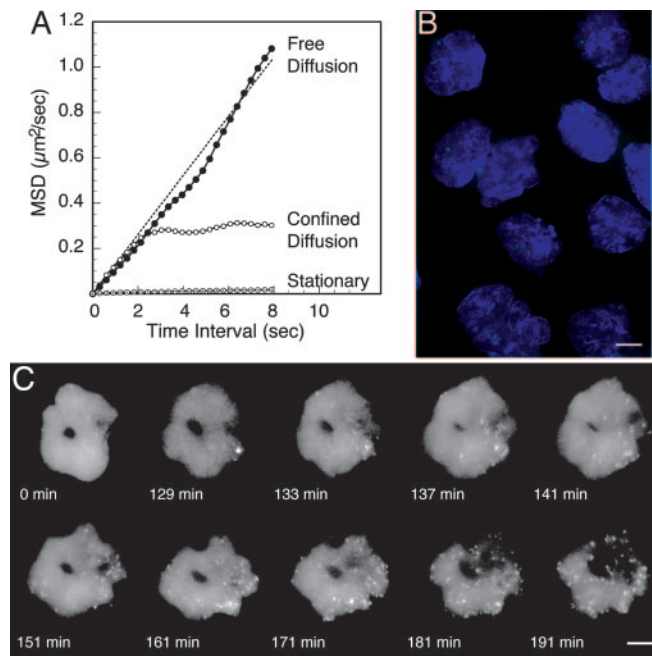
Fig. 3. Characterization of the diffusion of mRNA particles. (A) Relationship between the MSD of individual mRNA particles and the time interval during which the displacement occurred. Examples of three different types of behavior that were observed are shown. The dotted line indicates the results expected for freely diffusing particles with the average diffusion constant measured at 37°C. (B) Visualization of the locus of the gene that encodes the reporter mRNA. The image was obtained by in situ hybridization to cells whose DNA was denatured by heat and whose RNA was degraded by incubation with ribonuclease A by using a labeled oligonucleotide probe that is specific for the repeated sequence in the gene. The chromatin (stained with DAPI) is shown in blue, and the fluorescence of the probe is shown in green. (C) Dispersal of mRNA particles from the gene locus. Cells cultured in the presence of doxycycline to suppress the expression of the reporter mRNA were induced to express the reporter mRNA by the withdrawal of doxycycline while GFP-mRNA-96-mer was imaged. To view all of the particles, seven adjacent optical sections that were 0.2 \mu\text{m} apart were acquired for each time point and combined to form a single image. (Scale bars, 5 \mu\text{m} .)
